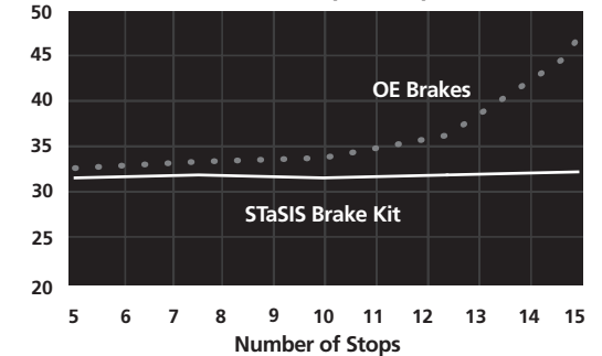
STOPPING DISTANCE OVER CONSECUTIVE STOPS FROM 100KPH (62MPH)
